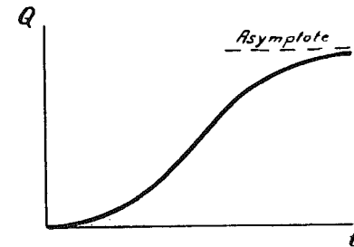
Fig. 3.4. Logistic curve.
